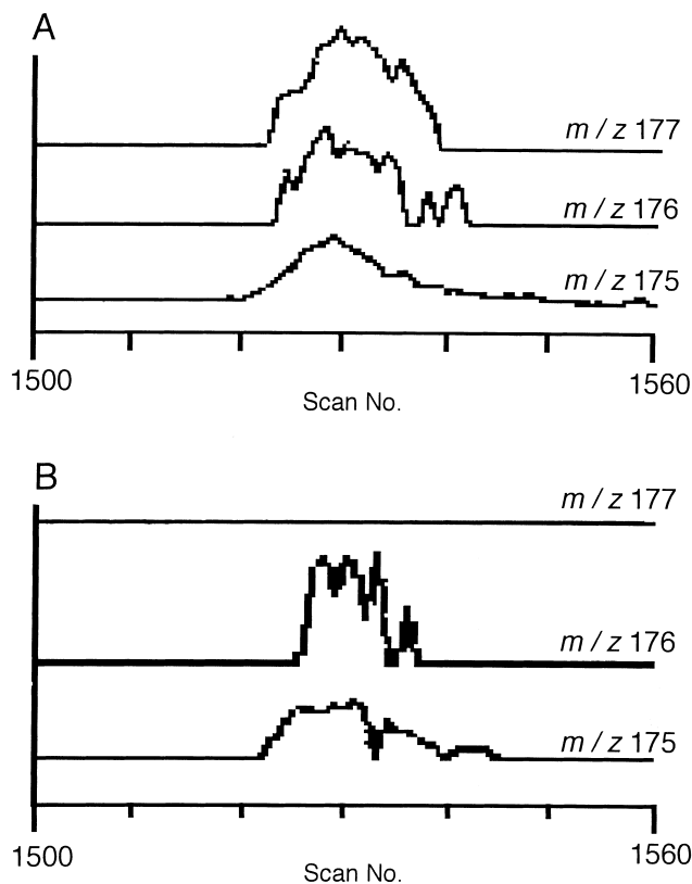
Fig. 6. Segments of GC-MS ion chromatograms of 7-hydroxycalamenene ( m/z 175–177) incorporating [\text{H}_2] -cubenene 17 (a) and without cubenene 17 (b).
