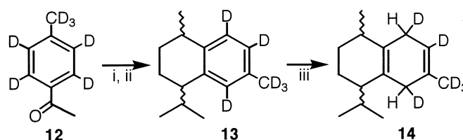
Fig. 3. Synthesis of [ ^2\text{H}_6 ]-calamenene ( 13 ) and its Birch reduction product ( 14 ): (i) 1-bromo-4-methyl pentane, Mg, 0°C (36%); (ii) \text{P}_2\text{O}_5 , 120°C (54%); (iii) Li, ethylenediamine, EtOH, THF, 0°C (22%).
