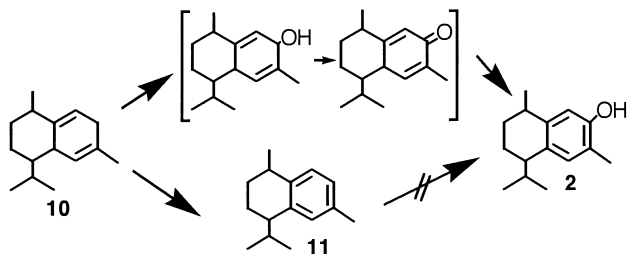
Fig. 7. Postulated biosynthesis of 7-hydroxycalamenene from cubenene 10 in the suspension cultured cells of H. planus .
