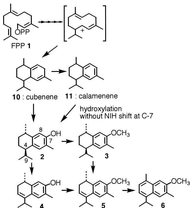
Fig. 1. Proposed biosynthesis of hydroxylated calamenenes and cadinenes from FPP in cultured cells of Heteroschypnus planus .
