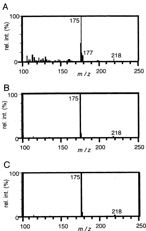
Fig. 5. Mass spectra of 7-hydroxycalamenene 2 synthesized in suspension cultured cells of H. planus fed with [\text{H}_2] -cubenene 17 (a), [\text{H}_6] -calamenene 13 (b) and without precursor (c).
