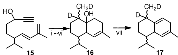
Fig. 4. Synthesis of [^2\text{H}_2] -cubenene ( 17 ): (i) Pyridinium chlorochromate, \text{CH}_2\text{Cl}_2 , room temp. (41%); (iii) m -chloroperbenzoic acid, \text{CH}_2\text{Cl}_2 , room temp. (41%); (iv) HF-pyridine, THF, 0^\circ\text{C} (79%); (v) methyltriphenylphosphonium bromide, NaH, DMSO, 0^\circ\text{C} (66%); (vi) \text{NaBD}_4 , \text{CoCl}_2 \cdot 6\text{H}_2\text{O} , \text{CD}_3\text{OD} , 0^\circ\text{C} (38%); (vii) \text{SOCl}_2 , pyridine, 0^\circ\text{C} , then 10% \text{NaHCO}_3 (56%).
