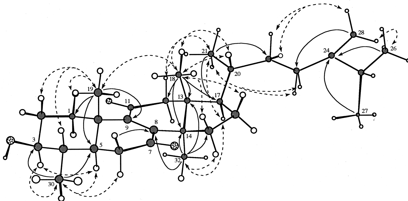
Fig. 2. HMBC (plain arrow) and selective NOESY (dashed arrow) correlations of 4a .
