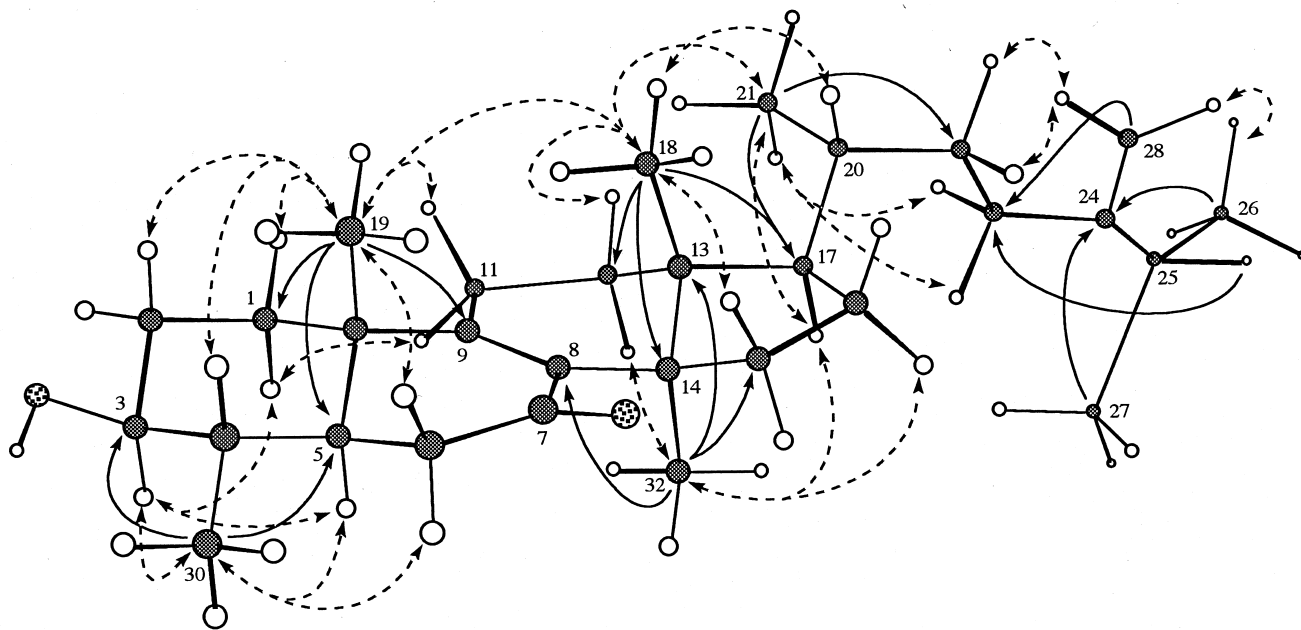
Fig. 1. HMBC (plain arrow) and selective NOESY (dashed arrow) correlations of 3a .
