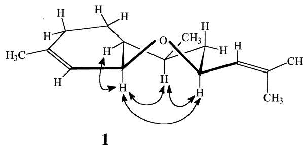
Fig. 1. NOE effects of bisabola-2,10-diene[1,9]oxide ( 1 ).
