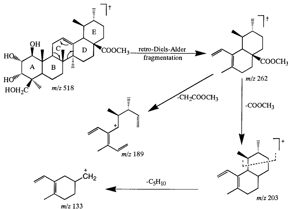
Fig. 1. Proposed EI mass spectral fragmentation of compound 1a .
