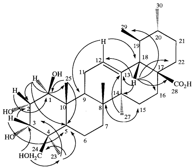
Fig. 2. Three and two-bond correlations for compound 1 in the HMBC spectrum.
