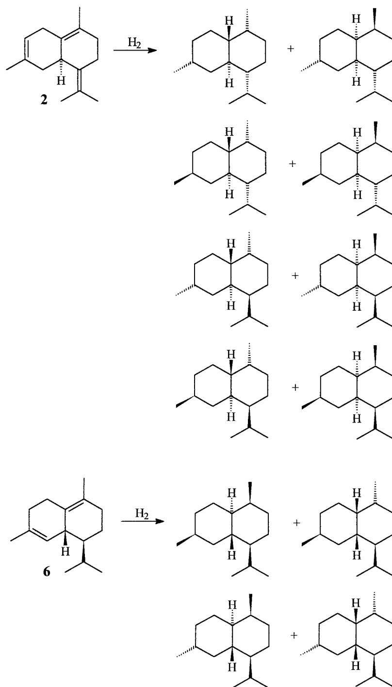
Fig. 4. Hydrogenation of (+)-Cadina-1(10),3,7(11)-triene (2) and (+)-δ-cadinene (6).
