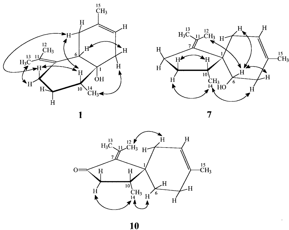
Fig. 2. NOE effects of 10β( H )-muurola-3,7(11)-dien-1-ol ( 1 ), α-alasken-6β-ol ( 7 ) and α-alasken-8-one ( 10 ).
