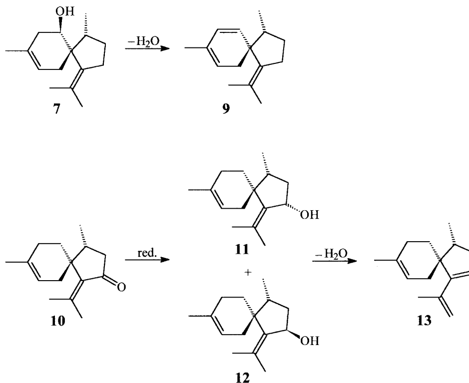
Fig. 5. Dehydration of (-)- \alpha -alasken-6 \beta -ol ( 7 ) to 5,6-dehydro- \alpha -alaskene ( 9 ) and reduction of (-)- \alpha -alasken-8-one ( 10 ) to \alpha -alasken-8 \alpha -ol ( 11 ) and \alpha -alasken-8 \beta -ol ( 12 ) and dehydration to 7,8-dehydro- \alpha -acoradiene ( 13 ).
