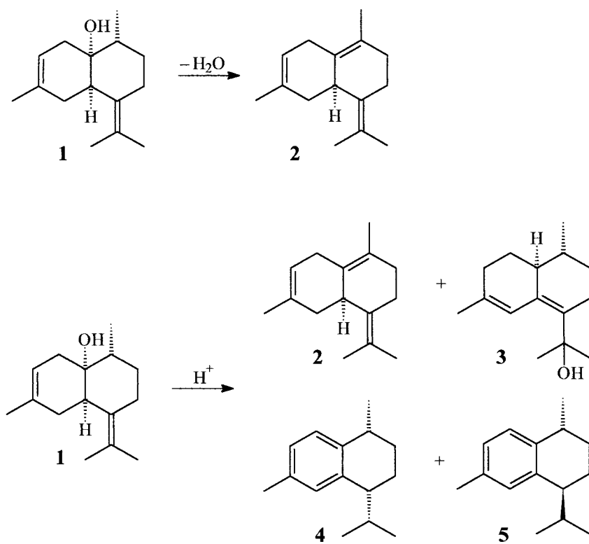
Fig. 3. Dehydration of (+)-10β( H )-muurola-3,7(11)-dien-1-ol ( 1 ) to (+)-cadina-1(10),3,7(11)-triene ( 2 ) and acid rearrangement of ( 1 ) to (+)-cadina-1(10),3,7(11)-triene ( 2 ), (+)- cis -cadina-4,6-dien-11-ol ( 3 ), (+)- cis -calamenene ( 4 ) and (-)- trans -calamenene ( 5 ).
