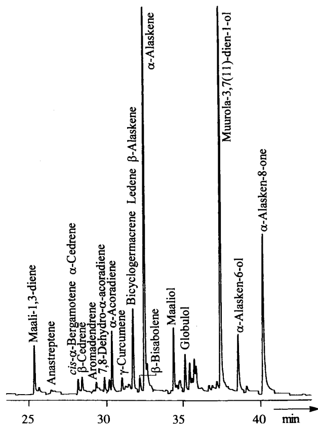
Fig. 1. Gas chromatogram of the essential oil of C. fissa on a 25 m fused silica capillary with polysiloxane CpSil5; column temp. 50°C, temp. program 3°/min to 230°C; carrier gas 0.5 bar H 2 .
