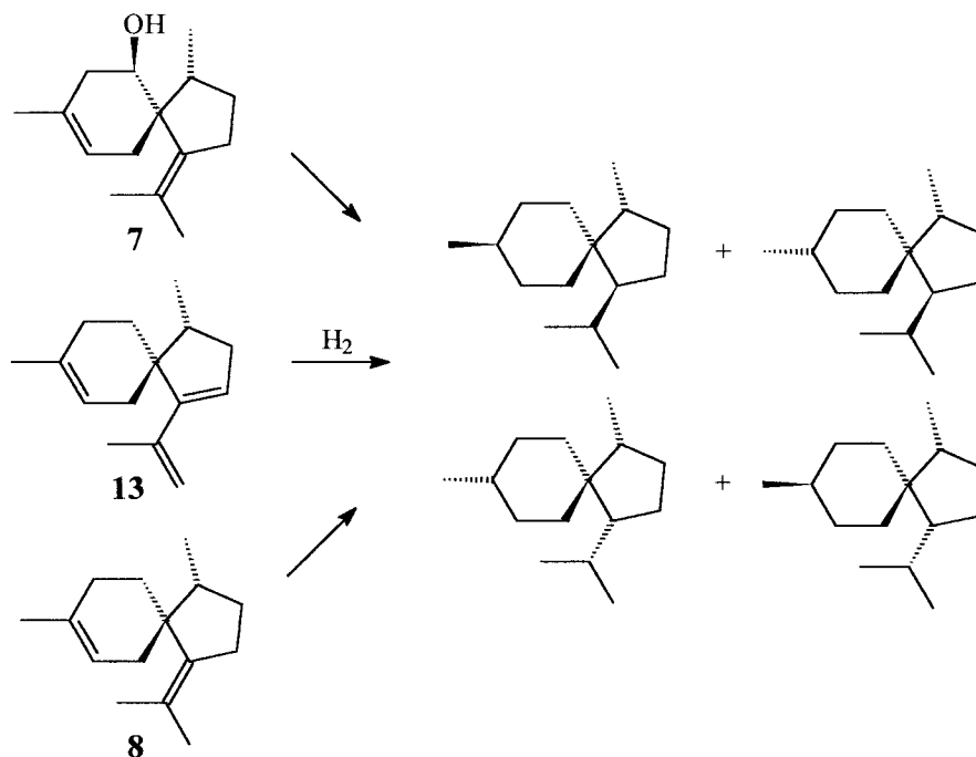
Fig. 6. Hydrogenation of (–)- \alpha -alasken-6 \beta -ol ( 7 ), 7,8-dehydro- \alpha -acoradiene ( 13 ) and (–)- \alpha -alaskene ( 8 ).
