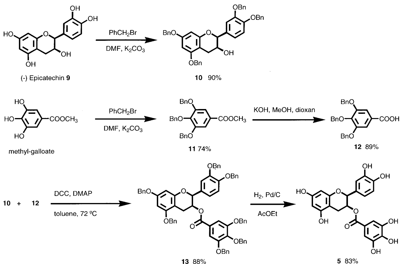
Scheme 1. Synthesis of (-) epicatechin-3- O -gallate.
