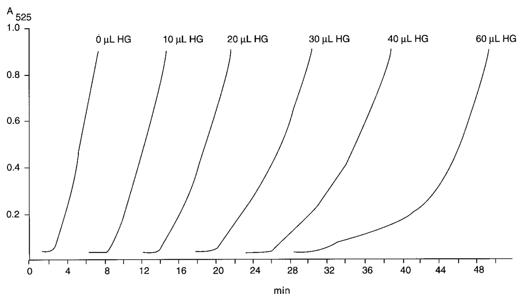
Fig. 1. Effect of HG on the enzymatic oxidation of SYR by C. hirsutus laccase. C. hirsutus , 20 \mu l, laccase (1 mg solid/ml; 1 mg protein/ml) was incubated with 0.2 ml of 0.5 mM SYR (0.1 \mu mole) and 1.8 ml of acetate buffer (pH 5.0). Various amounts (0.05 \mu mole/10 \mu l) of 5 mM HG dissolved in acetate buffer were added at zero time. Rates of the individual reactions at 525 nm were determined in A/min between 0 and 0.2 A and 0.6 to 0.9 A.
