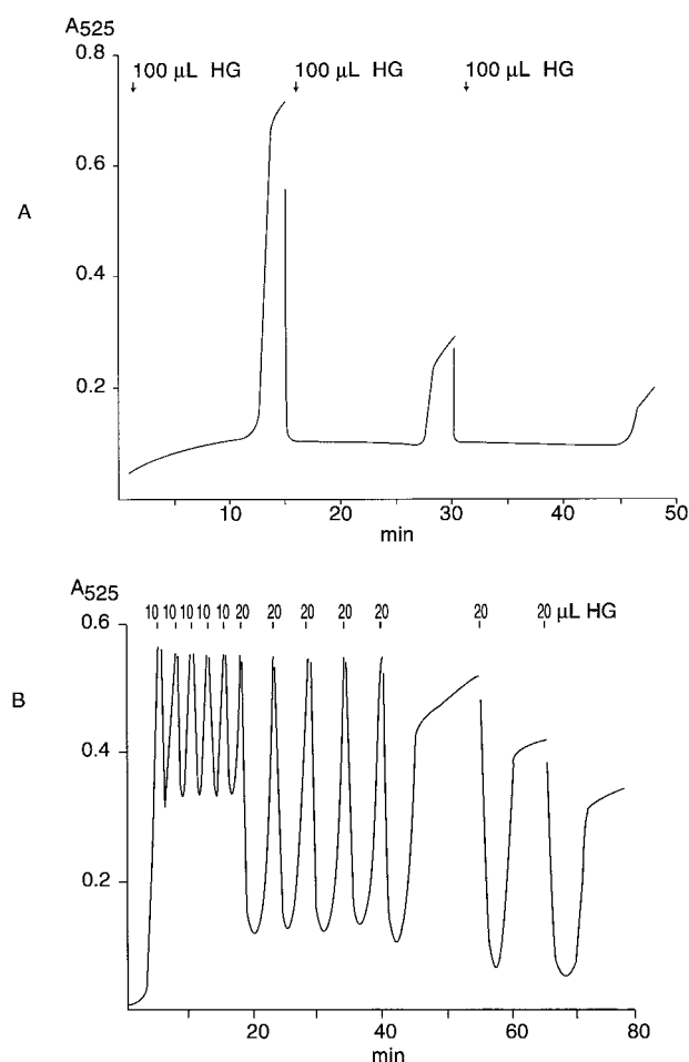
Fig. 2. Effect of HG on spectrophotometric enzyme assays monitoring the oxidation of SYR by C. hirsutus laccase. (A) 25 \mu L of C. hirsutus laccase (1 mg solid/ml; 1 mg protein/ml) was incubated with 0.1 ml of 0.5 mM SYR (0.05 \mu mole), 1.8 ml of acetate buffer and 0.1 ml of 5 mM HG (0.5 \mu mole) dissolved in acetate buffer. After the absorbance increased and began to taper off, a second aliquot of 5 mM HG was added. This process was repeated a third time. (B) 10 \mu L of C. hirsutus laccase was added to 1.8 ml acetate buffer and 0.1 ml of 0.5 mM SYR (0.05 \mu mole) and the absorbance monitored with time. The absorbance was allowed to increase to approximately 0.55 A, at which time 10 \mu L of 5 mM HG (0.05 \mu mole/10 \mu L) was added. The process was repeated several times with 10 and 20 \mu L additions of HG.
