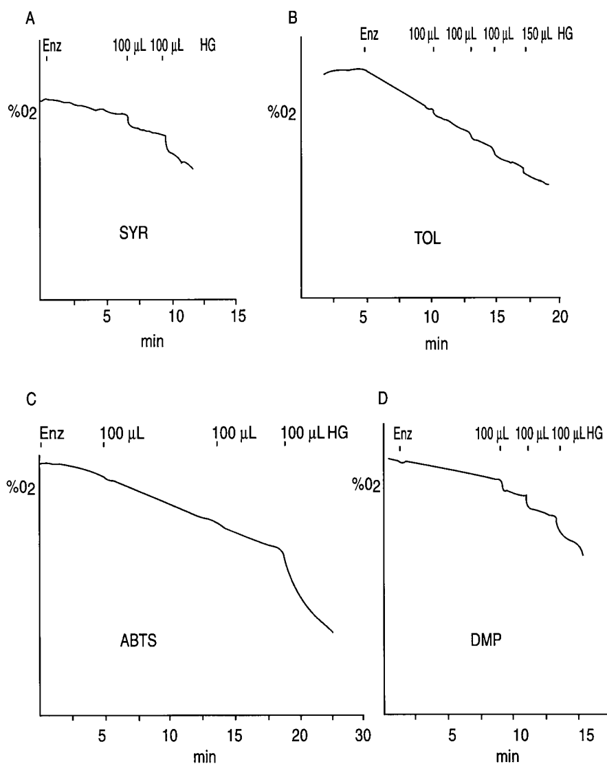
Fig. 3. Effect of HG on enzymatic oxygen uptake assays for laccase with different substrates. (A) 0.1 ml of SYR (0.1 \mu mole), 3.9 ml of acetate buffer, and 30 \mu l of A. bisporus laccase (2 mg protein/ml) were mixed in the electrode cell. Indicated amounts of 5 mM HG (0.5 \mu mole/0.1 ml) were added at the designated times. (B) 25 \mu l of 40 mM toluidine (1 \mu mole), 3.85 ml of acetate buffer, and 30 \mu l of A. bisporus laccase were mixed in the electrode cell. At the times indicated, specified amounts of 10 mM HG (1 \mu mole/0.1 ml) were added. (C) 3.6 ml of 0.5 mM ABTS (1.8 \mu mole) in acetate buffer and 30 \mu l of A. bisporus laccase were mixed in the electrode cell. At indicated times, 0.1 ml of 10 mM HG (1 \mu mole) was added. (D) 0.2 ml of 5 mM DMP (1 \mu mole) in acetate buffer, 3.6 ml of acetate buffer, and 10 \mu l of A. bisporus laccase were mixed in the electrode cell. At selected intervals, 0.1 ml of mM HG (0.5 \mu mole) was added. Oxygen uptake was followed with time using a Clark oxygen electrode.
