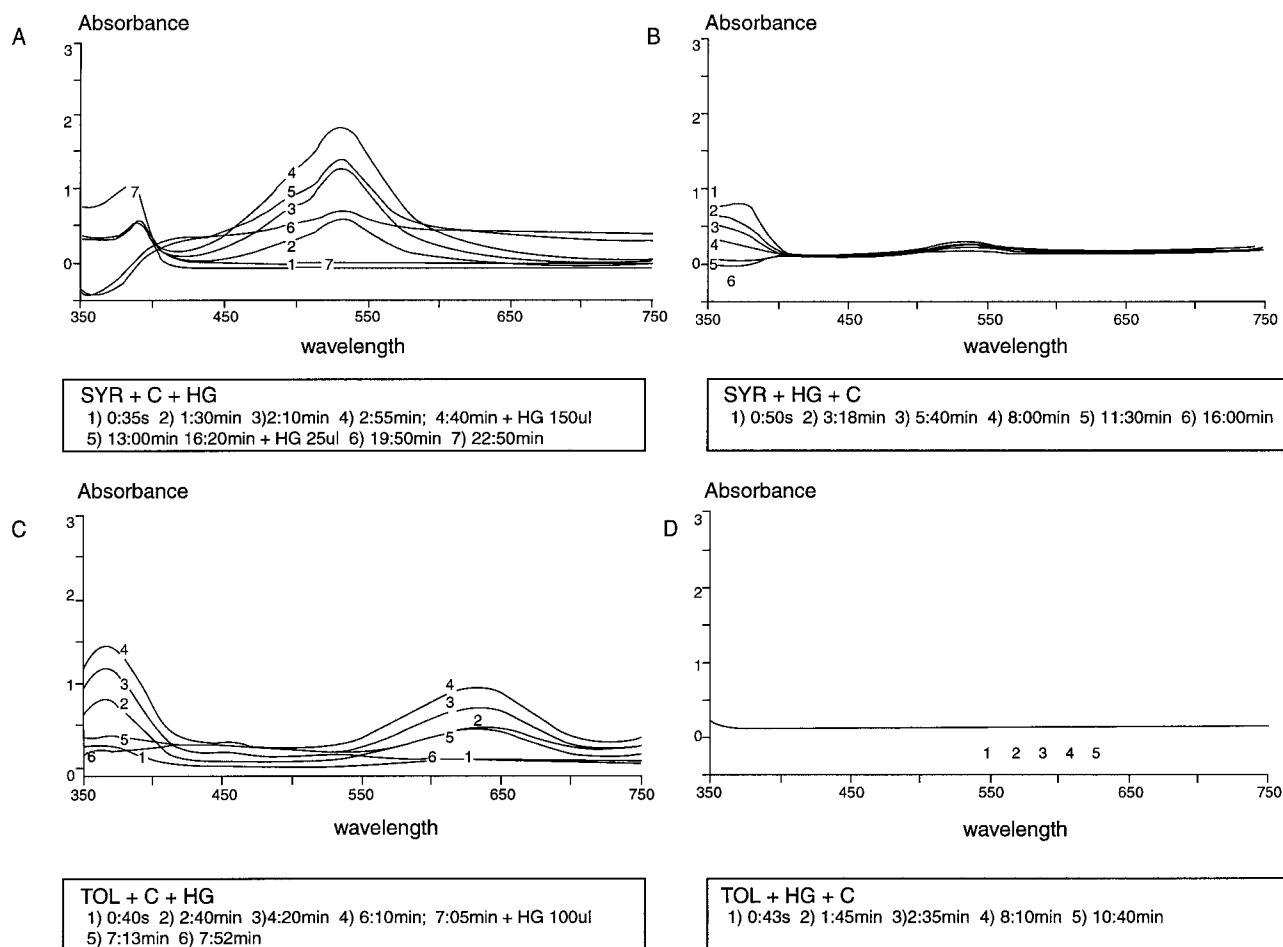
Fig. 4. Effect of HG on the absorption spectra of substrates oxidized enzymatically by laccase. HG (final concentration 1.25 mM) was added to buffer containing SYR (final concentration 0.17 mM) at time zero (B) or after the reaction was initiated with C. hirsutus laccase (A). HG (final concentration 1.0 mM) was added to buffer containing TOL (final concentration 2.0 mM) at time zero (D) or after the reaction was initiated with C. hirsutus laccase (C). HG (final concentration 0.91 mM) was added to buffer containing ABTS (final concentration 1.8 mM) at time zero (F) or after the reaction was initiated with C. hirsutus laccase (E). HG (final concentration 1.54 mM) was added to buffer containing DMP (final concentration 1.54 mM) at time zero (H) or after the reaction was initiated with C. hirsutus laccase (G). Spectral scans were carried out at time intervals indicated in the boxes.
