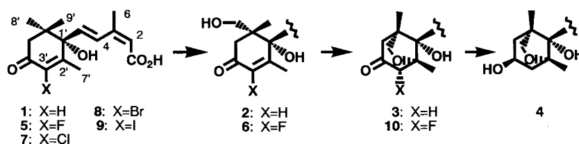
Fig. 1. Metabolic pathway of 1 and 5 , and structures of 7–9 .
