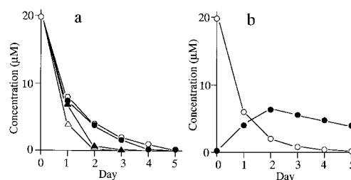
Fig. 3. Changes in concentrations of 1 and 7–9 (a) and of 5 and 6 (b) in the culture media. (a) ○, 1 ; ●, 7 ; △, 8 ; ▲, 9 . (b) ○, 5 ; ●, 6 .
