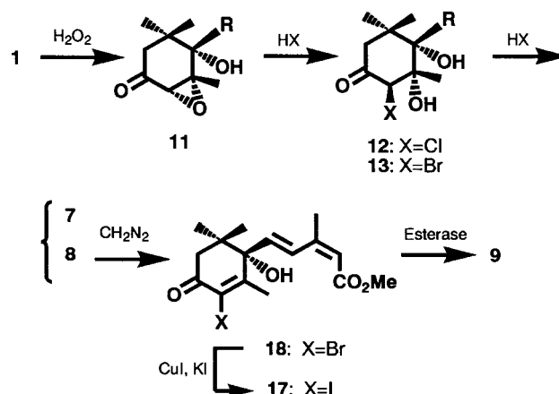
Fig. 2. Synthesis of (+)-3'-halo-ABAs, 7–9 . R is the side chain of 1 .
