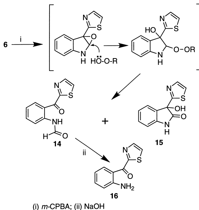
Scheme 3. Oxidation of camalexin ( 6 ) with m -chloroperbenzoic acid ( m -CPBA).
