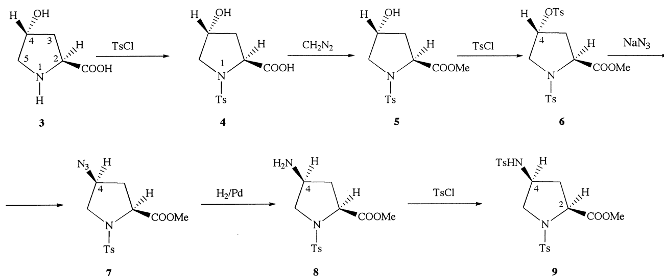
Fig. 1. Synthesis of N 1 , N 4 -ditosyl- cis -4-amino-L-proline methyl ester.
