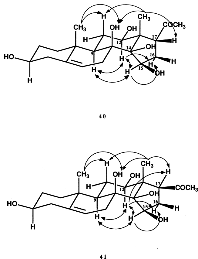
Fig. 1. Observed NOE correlations in compounds 40 and 41 .
