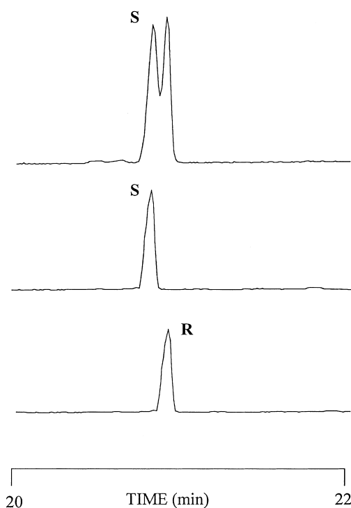
Fig. 2. Partial gas chromatogram (carbowax) indicating separation of C-22 diastereomers of HBI triene (II) isolated from different cultures of Haslea ostrearia . Chromatographic conditions are given in the text.
