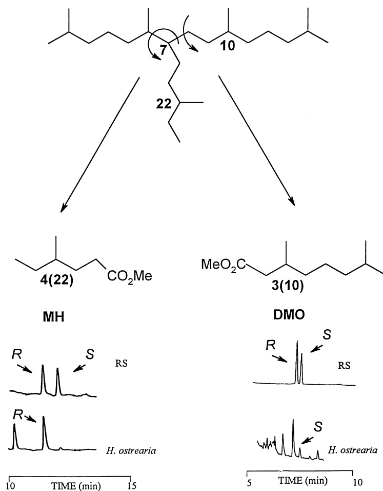
Fig. 1. Enantioselective (cyclodextrin) gas chromatography of HBI alkane oxidation products. Chromatographic conditions: (MH) octakis (6- O -methyl-2,3-di- O -pentyl)- \gamma -cyclodextrin (50% in polysiloxane OV 1701, wt./wt.) 50°C, isothermal, hydrogen carrier gas, 0.5 bar inlet pressure; (DMO) 2,6- O -dimethyl-3- O -pentyl- \beta -cyclodextrin, (50% in OV 1701, wt./wt.) 95°C hydrogen carrier gas, 0.5 bar inlet pressure.
