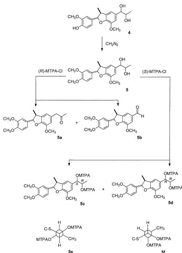
Scheme 1. Chemical transformations of 4 and 5 .
