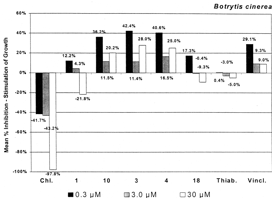
Fig. 3. Antifungal activity of compounds 1 , 10 , 3 , 4 , and 18 against Botrytis cinerea growth. Commercial standard fungicides: Chl. : chlorothalonil, Thiab. : thiabendazole, VincI. : vinclozolin. Least Square Means for percent inhibition of each sesquiterpene lactone is listed for each of three concentrations ( n = 4 ) by fungal species. Positive values indicate growth stimulation and negative values indicate growth inhibition relative the untreated control ( n = 32 ).
