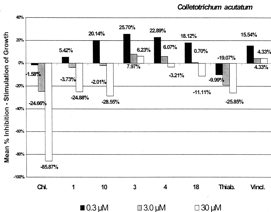
Fig. 4. Antifungal activity of compounds 1 , 10 , 3 , 4 , and 18 against Colletotrichum acutatum growth. Commercial standard fungicides: Chl. : chlorothalonil, Thiab. : thiabendazole, VincI. : vinclozolin. Least Square Means for percent inhibition of each sesquiterpene lactone is listed for each of three concentrations ( n = 4 ) by fungal species. Positive values indicate growth stimulation and negative values indicate growth inhibition relative the untreated control ( n = 32 ).
