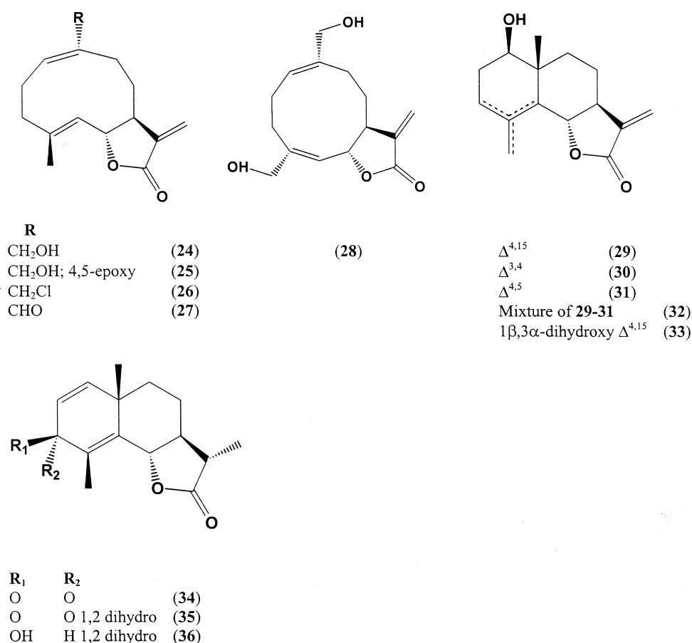
Fig. 2. Melampolides 24–27 , cis, cis -germacranolide 28 , and eudesmanolides 29–36 tested for antifungal activity.
