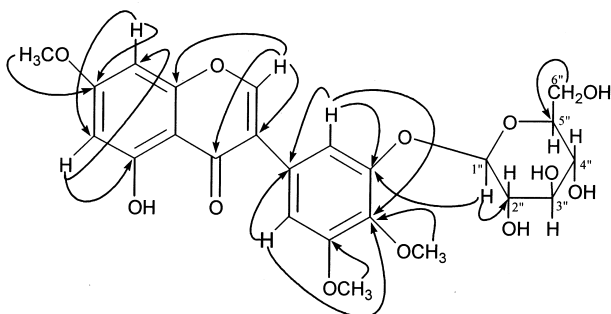
Fig. 3. Important HMBC interactions in Compound 2 .
