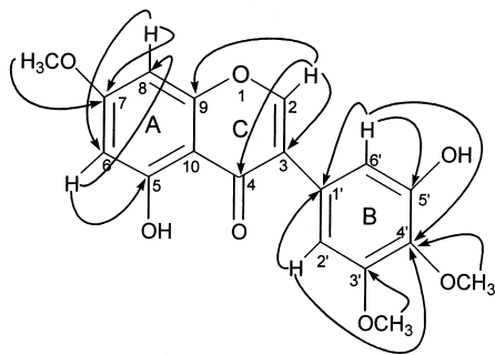
Fig. 1. Important HMBC interactions in Compound 1 .
