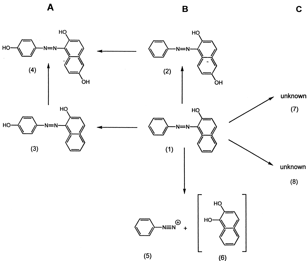
Fig. 2. Proposed metabolic scheme of Sudan I in the tulip CYP reconstituted system (A,B) and tulip peroxidase (B,C). (1) Sudan I; (2) 6-OH-Sudan I; (3) 4'-OH-Sudan I; (4) 4',6-di(OH)-Sudan I; (5) benzenediazonium ion; (6) 1,2-dihydroxynaphthalene; (7) unknown; (8) unknown. The metabolite in parentheses was not detected.
