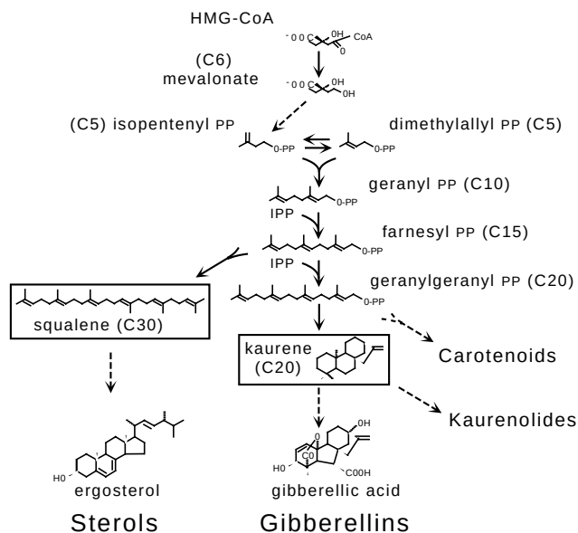
Fig. 1. Main steps in the biosyntheses of gibberellins and sterols in F. fujikuroi . Dotted arrows represent several reactions.
