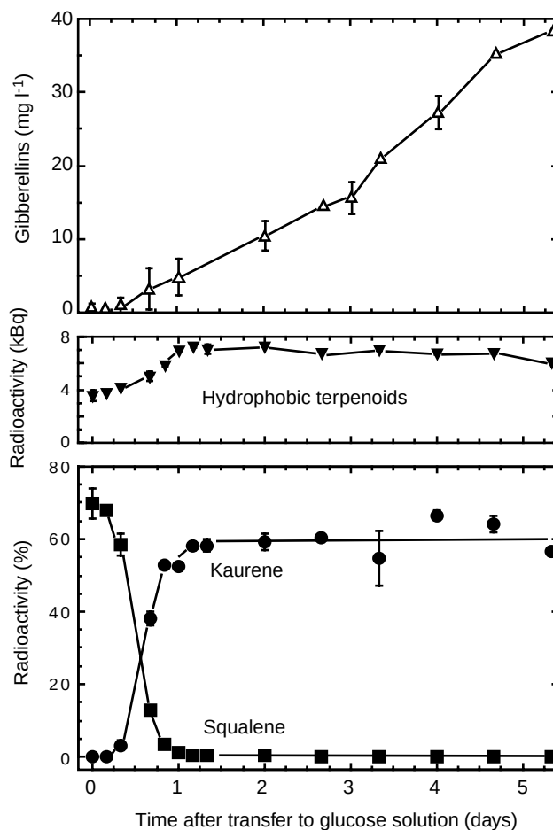
Fig. 5. Gibberellin production and in-vitro terpenoid biosynthesis after nitrogen deprivation. Mycelia grown for 6 days in high-nitrogen medium were transferred to a glucose solution. Upper panel, concentration of gibberellins in the solution. Central panel, total incorporation of radioactivity from [2\text{-}^{14}\text{C}]\text{mevalonate} into hydrophobic terpenoids. Lower panel, incorporation into kaurene (circles) and squalene (squares), as a fraction of total radioactivity into hydrophobic terpenoids.
