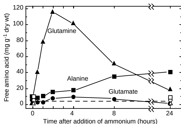
Fig. 4. Intracellular concentrations of free amino acids after addition of nitrogen source. \text{NH}_4\text{Cl} (final concentration 100 mM) was added (closed symbols) or not (open symbols and dashed line) to wild-type cultures grown for 8 days in low-nitrogen medium. Triangles, L-glutamine; squares, L-alanine; circles, L-glutamic acid.
