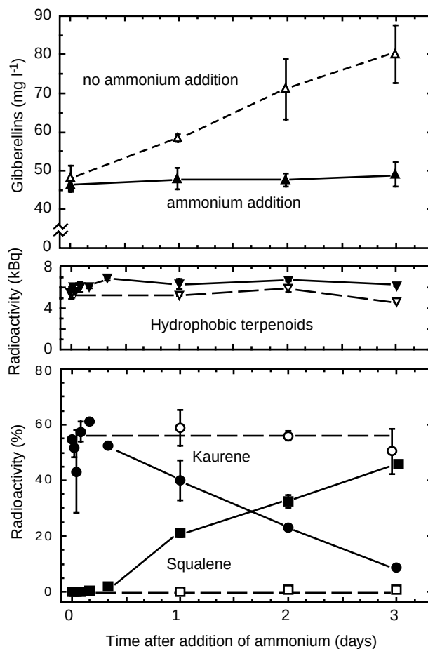
Fig. 3. Gibberellin production and in vitro terpenoid biosynthesis after addition of nitrogen source \text{NH}_4\text{Cl} (final concentration 100 mM) was added (closed symbols) or not (open symbols) to wild-type cultures grown for 8 days in low-nitrogen medium. Upper panel, concentration of gibberellins in the medium. Central panel, total incorporation of radioactivity from mevalonate into hydrophobic terpenoids. Lower panel, incorporation into kaurene (circles) and squalene (squares), as a fraction of total radioactivity in hydrophobic terpenoids.
