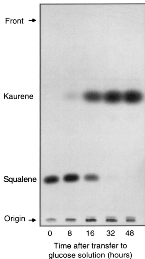
Fig. 7. Terpenoids synthesised from [2- 14 C]mevalonate by cell-free extracts from mycelia incubated in high-nitrogen medium for 6 days and in a glucose solution for the time indicated. Autoradiography of a TLC plate exposed on X OMAT S film (kodak) for 14 days.
