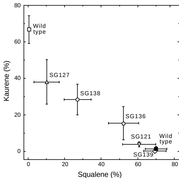
Fig. 2. Biosynthesis of terpenoids in cell-free extracts. Radioactivity in kaurene or squalene as a fraction of total radioactivity in hydrophobic terpenoids (2.1 kBq per experiment in the average) after the incubation of cell-free extracts from wild type and gib mutant mycelia with [2-^{14}\text{C}] mevalonate. Cultures were grown for 6 days in low-nitrogen medium (open symbols) or high-nitrogen medium (closed symbols).
