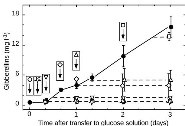
Fig. 6. Inhibition of gibberellin production by cycloheximide. Mycelia grown for 6 days in high-nitrogen medium were transferred to a glucose solution and cycloheximide was added at different times. Open symbols and dashed lines, concentration of gibberellins in the solution after cycloheximide addition at the time indicated by the arrows. Closed symbols and continuous lines, controls without cycloheximide.
