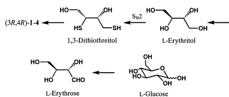
Fig. 1. Retrosynthesis of (1 S ,3 R ,4 R )- 1 .
