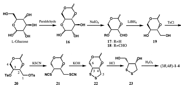
Fig. 2. Synthesis of (3 R ,4 R )- 1–4 .
