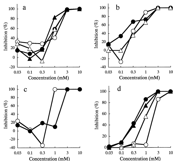
Fig. 3. Inhibitory activities of (3 R ,4 R )- 1–4 (a), of 5–7 (b), and of (3 R ,4 R )- 1–4 and (3 S ,4 S )- 23 (c) on root weight of rice seedlings, and of (3 R ,4 R )- 1–4 (d) on lettuce seed germination. (a) and (d) ○: 1 , ●: 2 , △: 3 , ▲: 4 ; (b) ○: 5 , ●: 6 , △: 7 ; (c) ○: (3 R ,4 R )- 23 , ●: (3 S ,4 S )- 23 .
