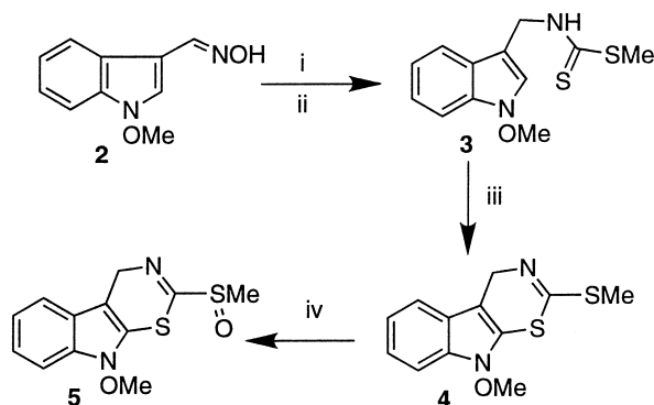
Scheme 1. (i) \text{TiCl}_3/\text{NaBH}_3\text{CN}/\text{NH}_4\text{Ac} ; (ii) \text{CS}_2/\text{Py}, \text{Et}_3\text{N} ; MeI, 60%; (iii) \text{CH}_2\text{Cl}_2/\text{NBS} , 41%; (iv) m -CPBA, 20%.
