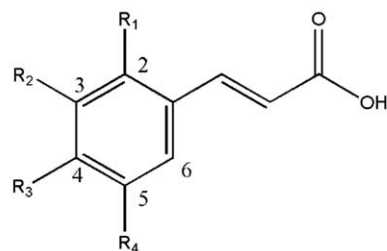
Cinnamic acids ( 17–21 )
