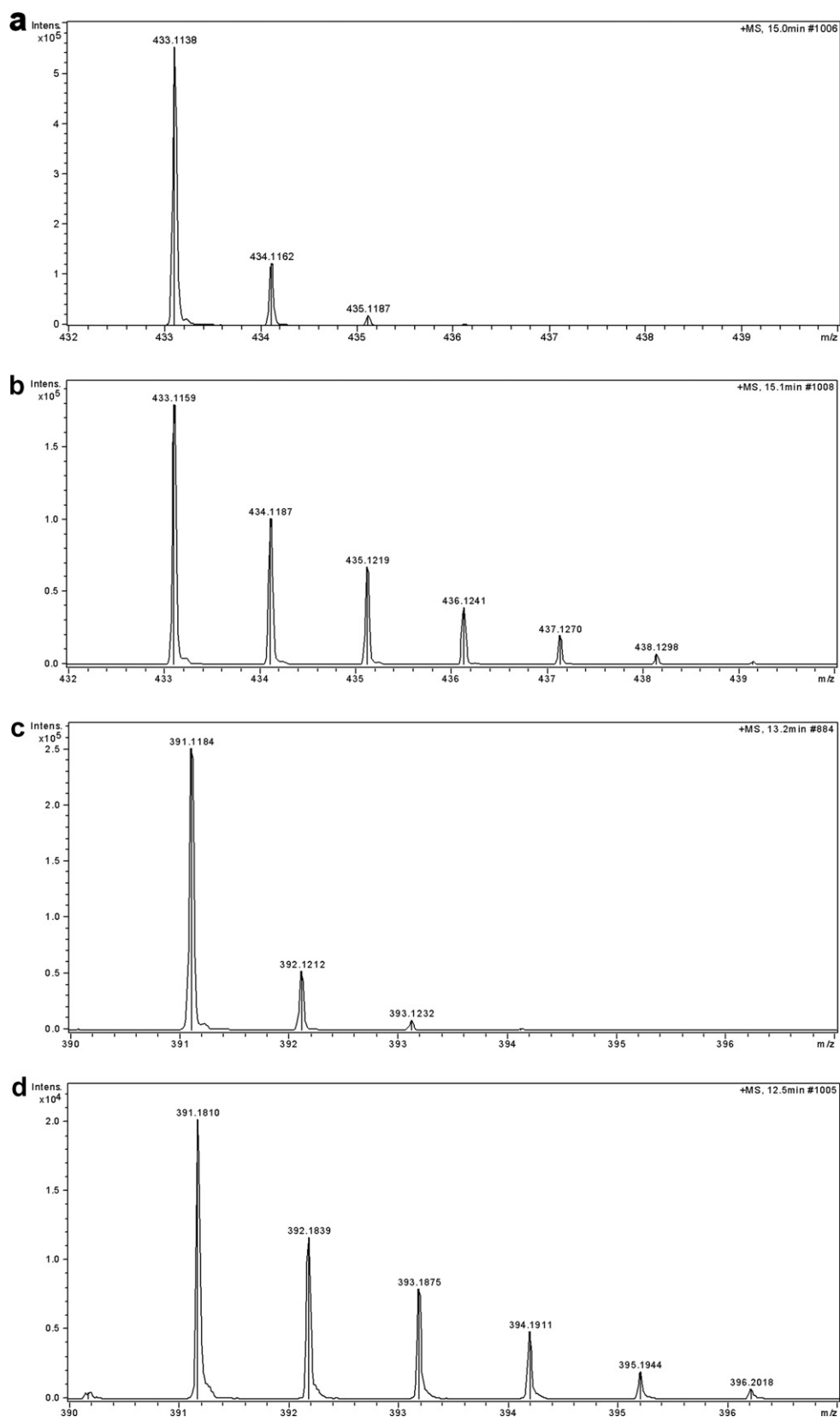
Fig. 3. Mass spectra showing incorporation of ^{13}\text{C} from the experiment with [2-^{13}\text{C}]\text{-glucose} . (a) standard of salvinorin A ( 1 ), (b) m/z 433.1159 [\text{M}+\text{H}]^+ refers to salvinorin A parent peak. Subsequent peaks form an isotope cluster reflecting the incorporation of ^{13}\text{C} into the molecule of 1 . (c) standard of salvinorin B ( 2 ), (d) m/z 391.1810 [\text{M}+\text{H}]^+ corresponds to 2 . Isotope cluster is spread to [\text{M}+5]^+ .
