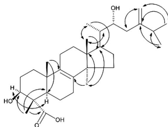
Fig. 3. Key correlations in HMBC (H→C) and NOESY (←→) spectra of 2 .
