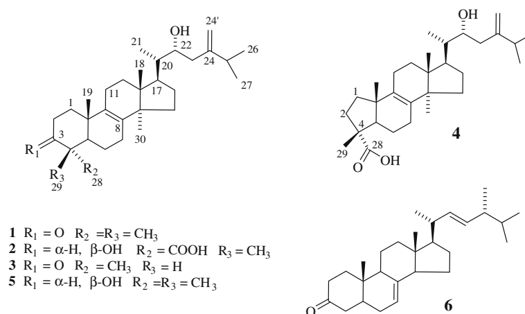
Fig. 1. Chemical constituents from Phyllinus gilvus .
