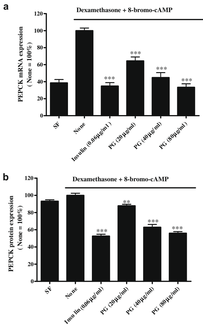
Fig. 4. Phellinus gilvus (PG) dose-dependent suppression of PEPCK mRNA and protein expression. (A) Semi-quantified effect of dexamethasone (500 nM) and 8-bromo-cAMP (100 \mu\text{M} ) induced PEPCK mRNA expression in presence or absence of ethanol–H 2 O (1:1) extract of Phellinus gilvus (PG-Et). Insulin (0.06 \mu\text{g/ml} ) served as the experimental control. Quantified data was presented as mean \pm SEM ( n = 4). *** P < 0.001 when compared with control (none). (B) Semi-quantified effect of dexamethasone (500 nM) and 8-bromo-cAMP (100 \mu\text{M} ) induced PEPCK protein expression in presence or absence of PG-Et or insulin (0.06 \mu\text{g/ml} ). Quantified data was presented as mean \pm SEM ( n = 4). ** P < 0.01 and *** P < 0.001 when compared with control (none).
