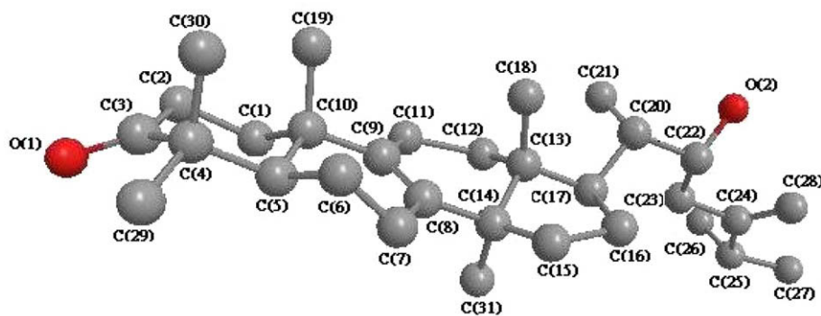
Fig. 2. 3-D structural drawing with atomic labeling of compound 1 . Hydrogen atoms are omitted for clarity.
