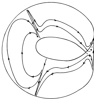
FIGURE 3 The Case X = P^2 (a)
