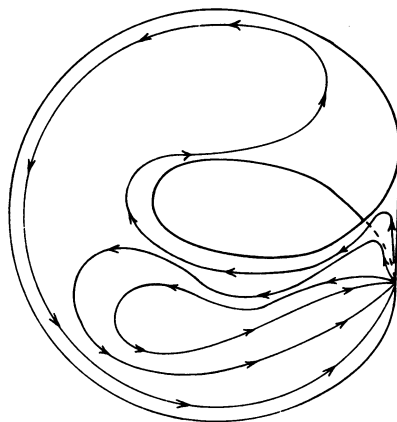
FIGURE 3 The Case X = P^2 (c)
