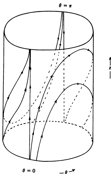
FIGURE 1 System (1)
