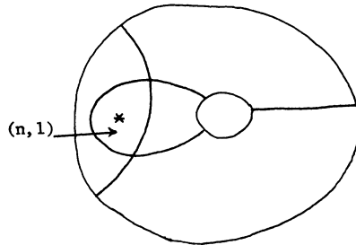
The Essential Arcs in the Orbit Manifold of L
