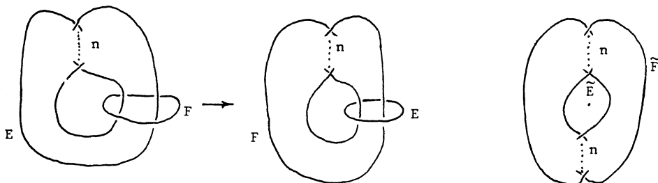
A Torus Link Exterior Double-covering V
