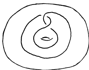
A Doubling Curve
