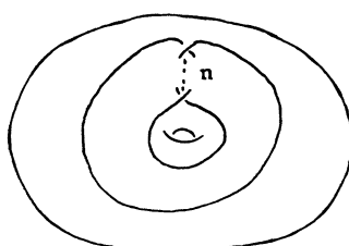
A Generalized Doubling Curve
