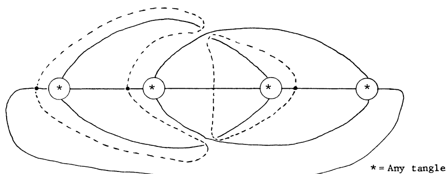
Alternate Configuration of a Separating Sphere
