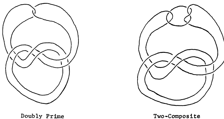
Satellites of the Trefoil with Embellishment the Unknot
