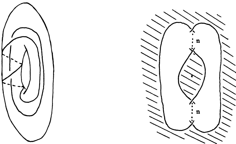
Visualizing the Essential Annuli in L
