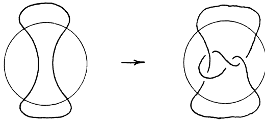
5/2 Untangle Surgery on the Unknot
