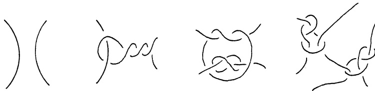
Tangles Which are Not Prime
