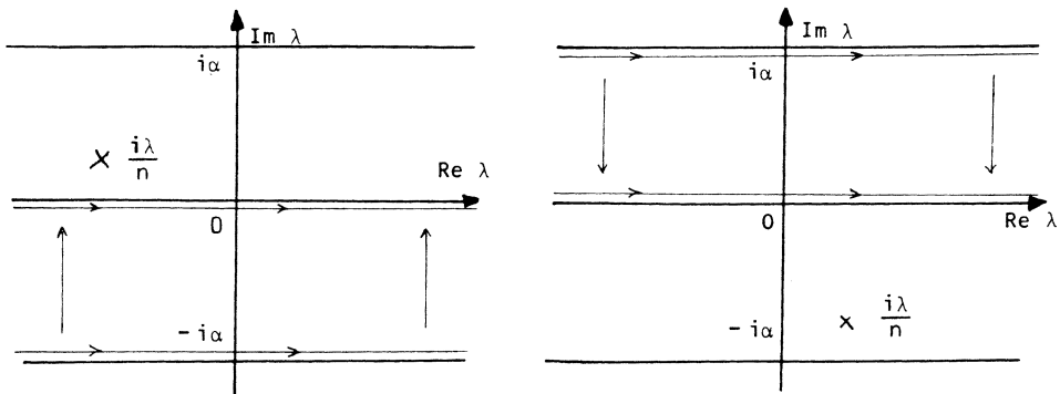
Case n > 0 \Rightarrow \operatorname{Im}(i\lambda/n) > 0 Deformation of the integration path from \operatorname{Im} \lambda = -\alpha to \operatorname{Im} \lambda = 0
