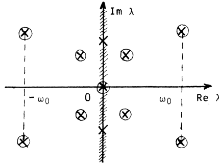
FIGURE 1. Spectrum of T . ( \times = Point spectrum; \circ = Residual spectrum;
