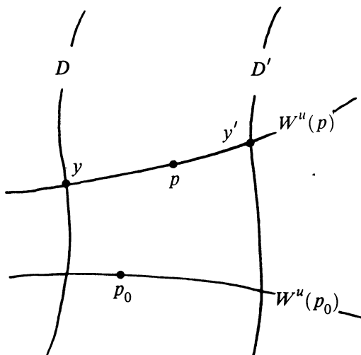
FIGURE 1. W^u -holonomy
