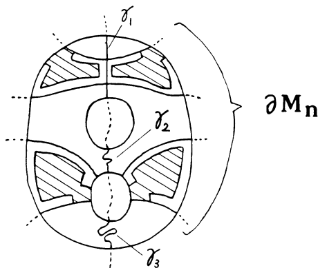
FIGURE 5. A cross section of (M'_k, a'_k) . The shaded area is X_{i_0} .
