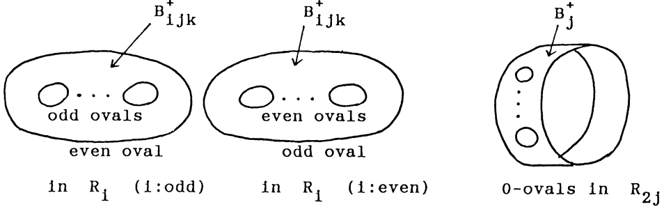
FIGURE 2.3. THE COMPONENTS OF B^+
