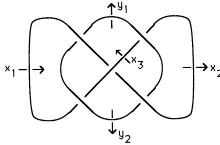
FIGURE 8. The Whitehead link WL
