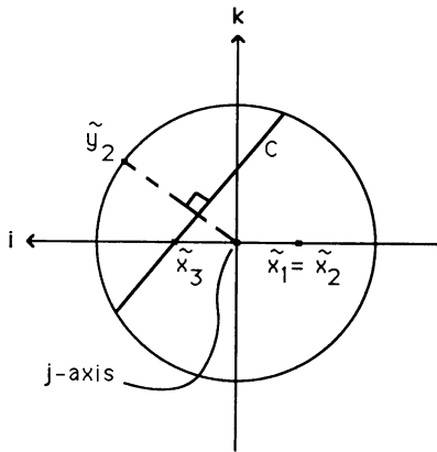
FIGURE 11. A projection of \Sigma_0 along the j -axis
