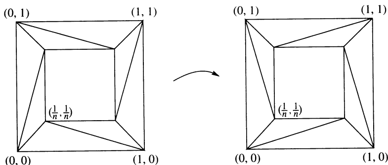
FIGURE 1. A “ \frac{1}{4} Dehn twist” in \text{Aut}_1(P, \partial)
