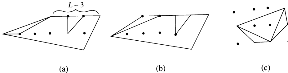
FIGURE 7. (a) Two inner triangles; (b) one inner, one side; (c) two side triangles (begin with the inner triangle, which contains all of \text{int } S \cap \mathbb{Z}^2 , and then add side triangles).
