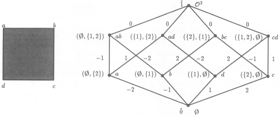
FIGURE 1. A standard labeling of \mathcal{C} .
