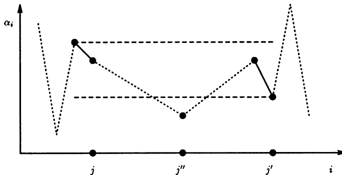
FIGURE 2. Condition (A_n) : the existence of j < j' such that \alpha_{j-1} > \alpha_j , \alpha_{j'-1} > \alpha_{j'} , \alpha_{j'} < \alpha_j , and \alpha_{j-1} > \alpha_{j'-1} implies the existence of j < j'' < j' so that \alpha_{j''} < \alpha_{j'} .
