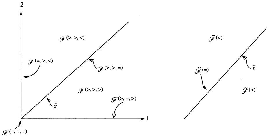
FIGURE 3. Facets of the modified join-the-shorter-queue model.
