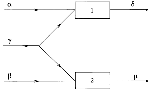
FIGURE 1. The modified join-the-shorter-queue model.
