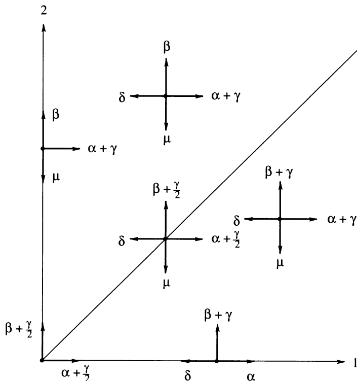
FIGURE 2. Jump intensities for the modified join-the-shorter-queue model.
