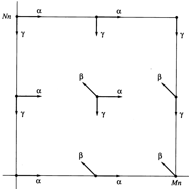
FIGURE 4. Jump intensities for the queueing system with finite buffers.
