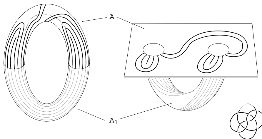
FIGURE 6. A presentation of -k_1
