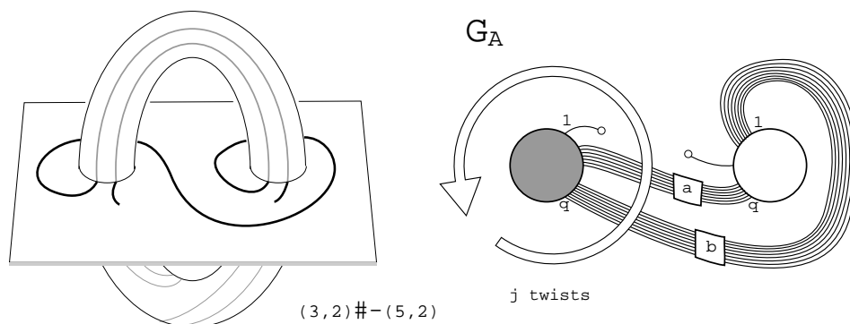
FIGURE 30. A \cup \partial V for (3,2) \# (5,-2) and G_A for (p,q) \# (p+q,-q)
