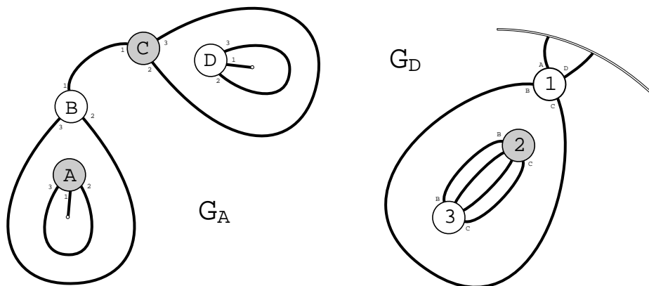
FIGURE 28. A pair of graphs that induces only an unknotted twisted unknot
