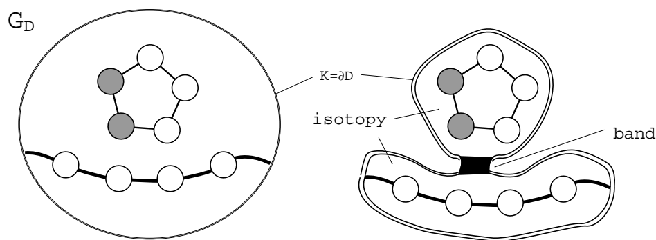
FIGURE 11. How a band sum arises from a multi-component G_D
