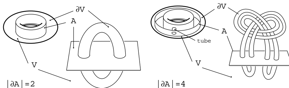
FIGURE 25. Possible splitting spheres in V
