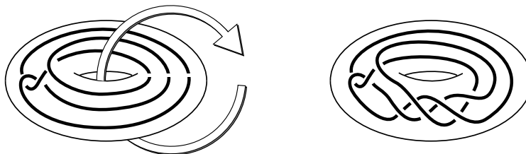
FIGURE 1. A twisting of a knot
