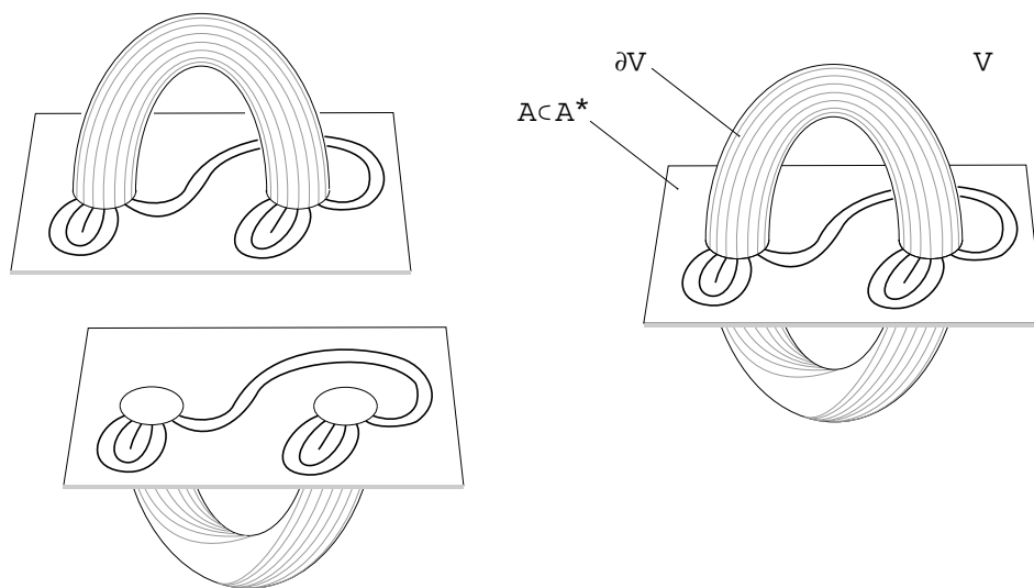
FIGURE 7. Joining the presentations of k and -k_1 to obtain A \cup \partial V
