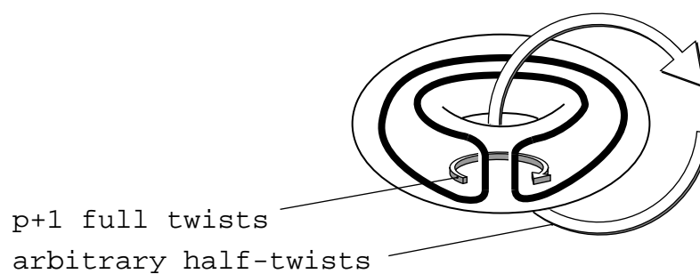
FIGURE 33. The pattern of a cosummand for (p, p+1)
