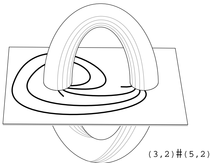
FIGURE 29. A \cup \partial V for (3, 2) \# (5, 2)
