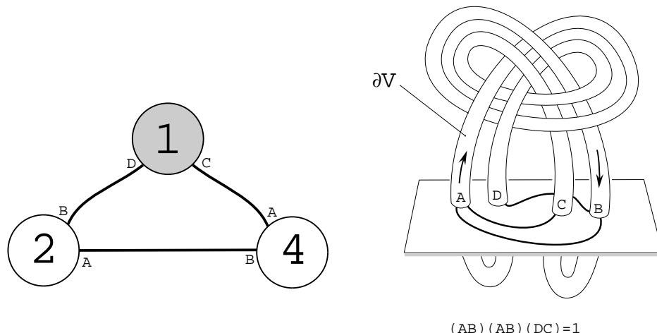
FIGURE 4. How the graphs provide relations in the homology
