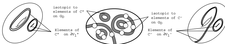
FIGURE 13. Elements of C^+ , and C^-
