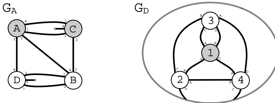
FIGURE 26. A pair of graphs of intersection with torsion but not all types
