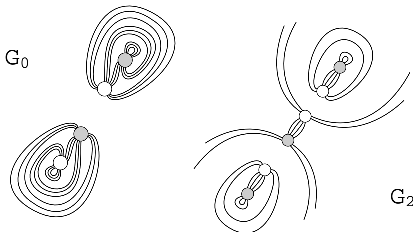
FIGURE 21. A pair of ring graphs
