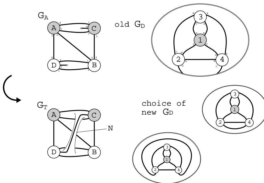
FIGURE 17. Constructing the new graphs of intersection
