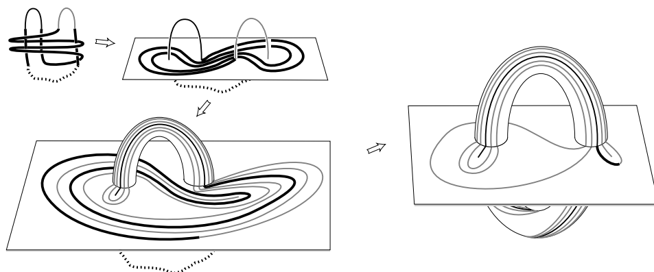
FIGURE 32. A \cup \partial V for the sum of a two-bridge knot and its reflection
