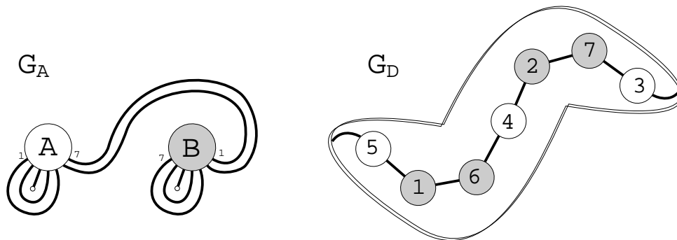
FIGURE 9. The graphs of intersection for our K = k \# (-k_1)
