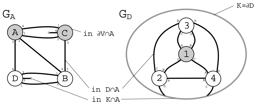
FIGURE 2. A pair of graphs of intersection
