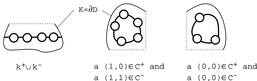
FIGURE 15. Pieces of G_D
