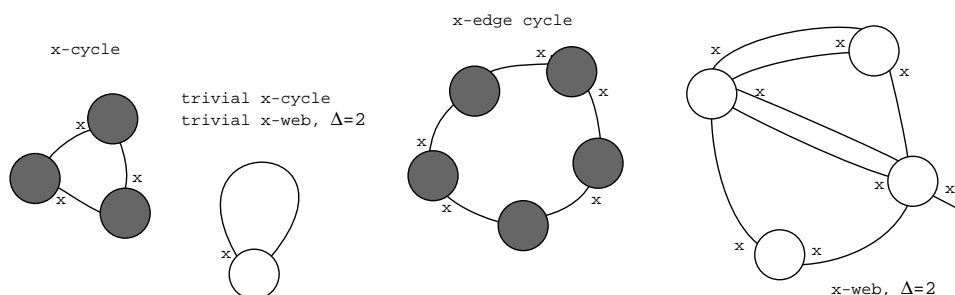
FIGURE 18. Various x -objects
