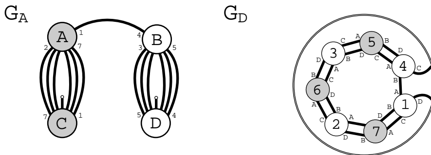
FIGURE 27. A pair of graphs containing klein bottles
