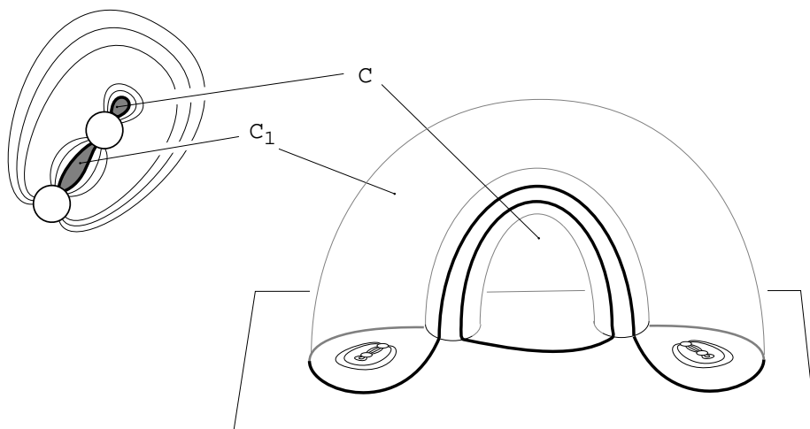
FIGURE 22. There are no bigons on the same label pair as a one-sided face
