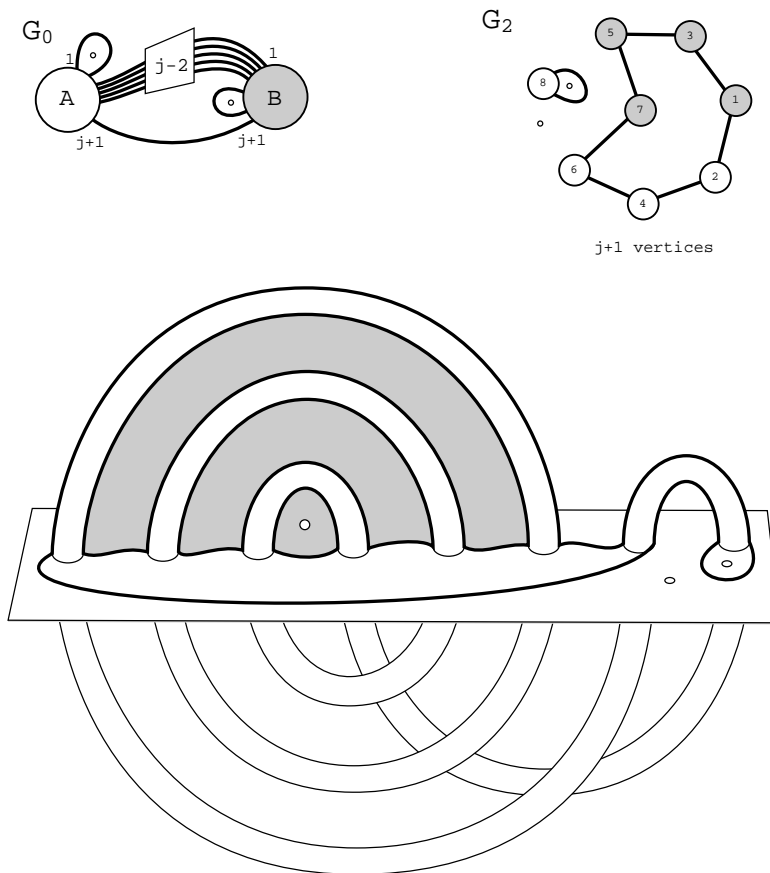
FIGURE 35. Graphs relating all composite K to all K_1 \# (j, 2)
