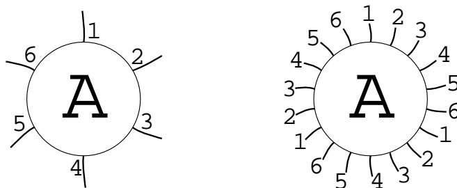
FIGURE 3. A fat vertex with \Delta = 1 and one with \Delta = 3
