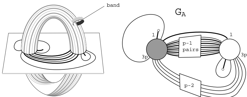
FIGURE 10. A \cup \partial V and G_A for one of Teragaito's examples
