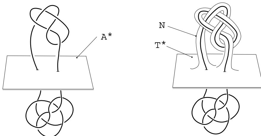
FIGURE 16. Creating a “swallow/follow” torus
