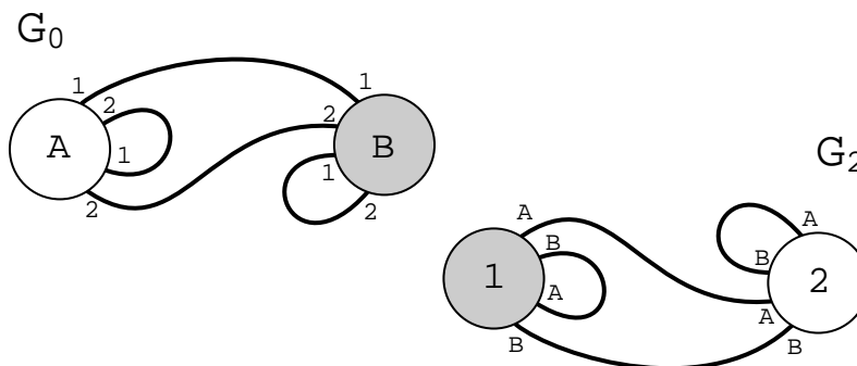
FIGURE 19. A pair of graphs which induce the granny knot
