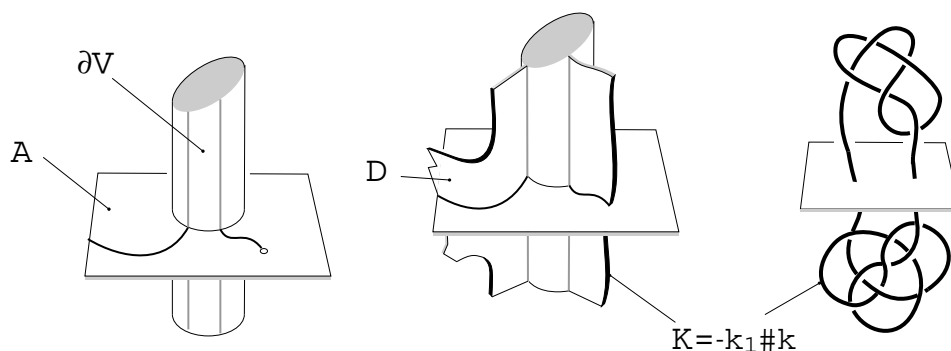
FIGURE 8. Isotoping the presentations of k and -k_1 to obtain K
