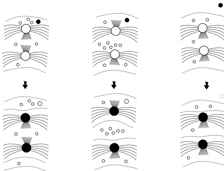
FIGURE 24. Partitioning loop annuli
