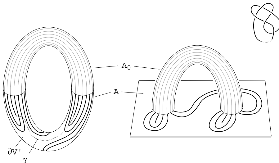
FIGURE 5. A presentation of a torus one-bridge knot k
