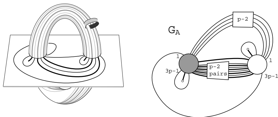
FIGURE 34. A \cup \partial V and G_A for another banded example
