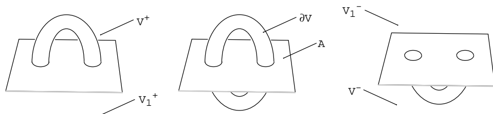
FIGURE 12. V^+ , V^- , V_1^+ , and V_1^-
