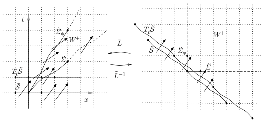
FIGURE 4.1. The Straightening Conjugacy. (Here, \mathbf{p}/\mathbf{q} = 4/5 and \mathbf{p}_*/\mathbf{q}_* = 3/4 .)
