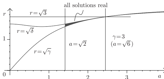
FIGURE 2. Discriminant locus and values of a, r giving all solutions real
