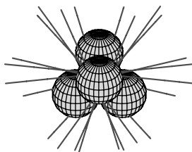
FIGURE 1. Spheres with 12 real common tangents
