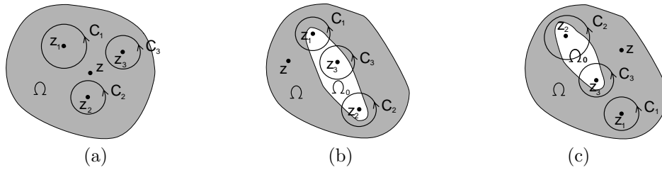
FIGURE 3. Integration contours \mathcal{C}_k for p = 3 and q = 1 .
