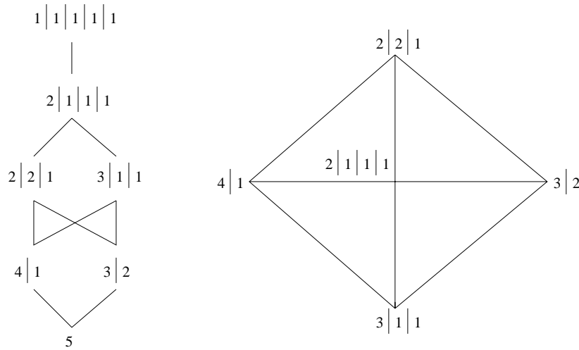
FIGURE 5. \Pi_5/S_5 and its (2-dimensional) order complex \Delta(\Pi_5/S_5)
