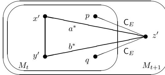
FIGURE 1. The network M_{t+1}
