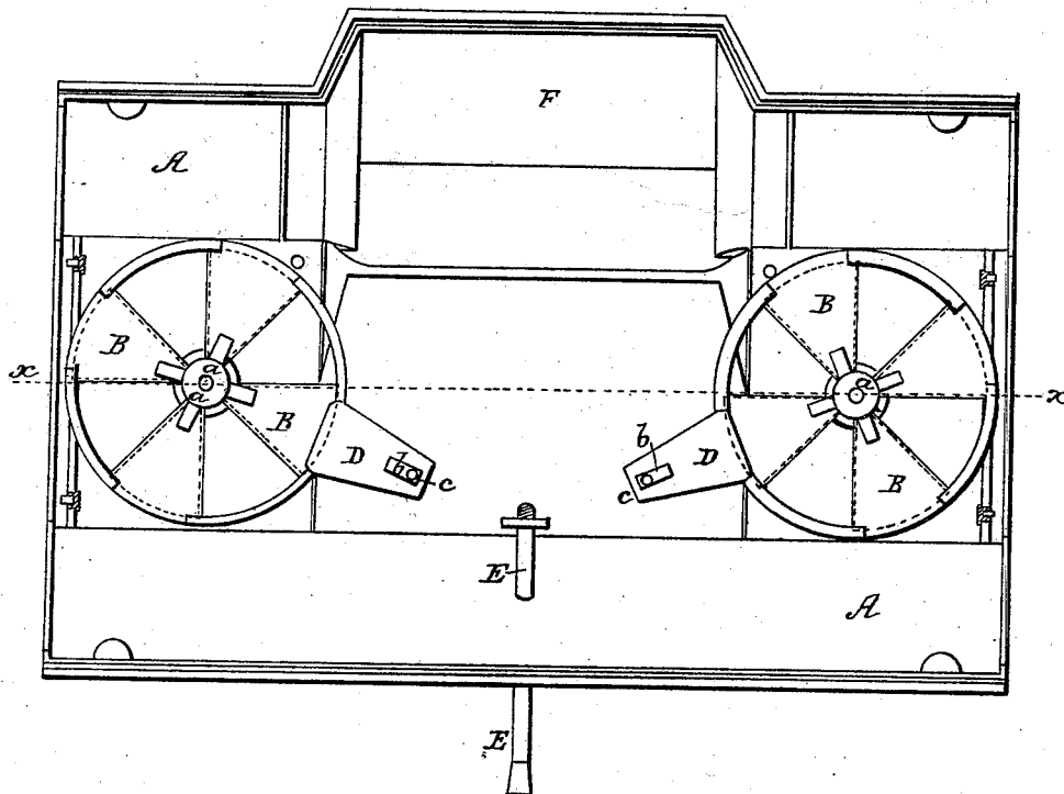
Fig. 2 Sectional View.
