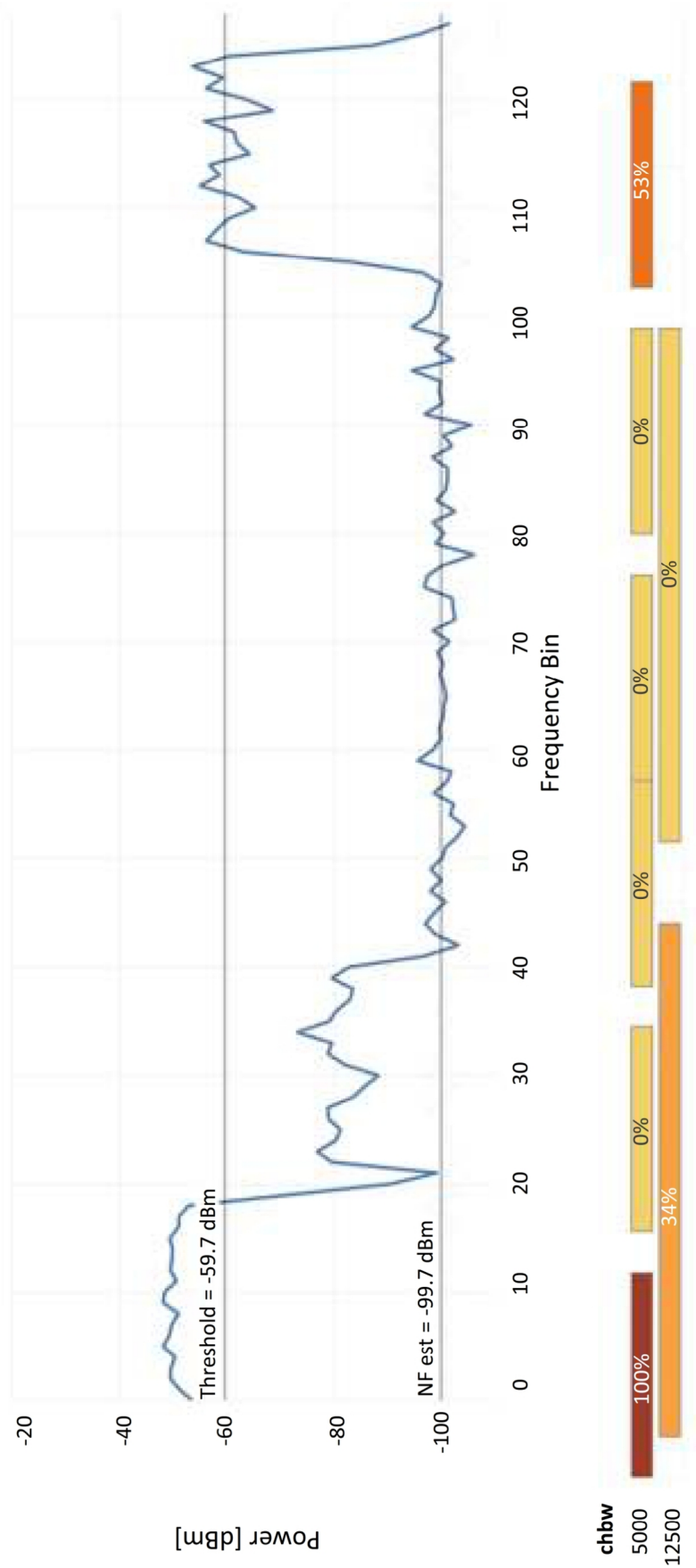
FFT Frame #1
