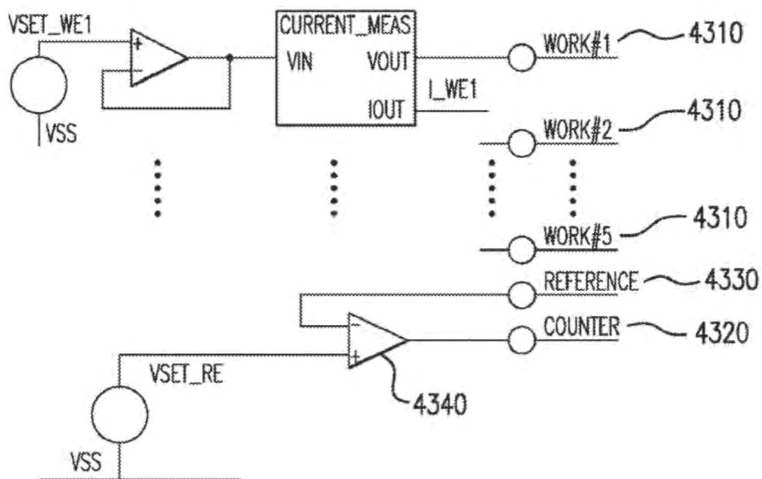
POTENTIOSTAT CONFIGURATION
